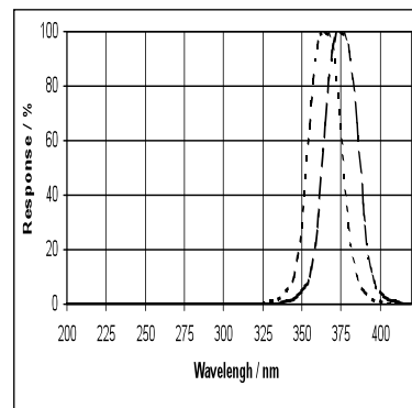
UV LEDs Spectral Emissions (dots - 365nm peak) (dashes - 375nm peak)
